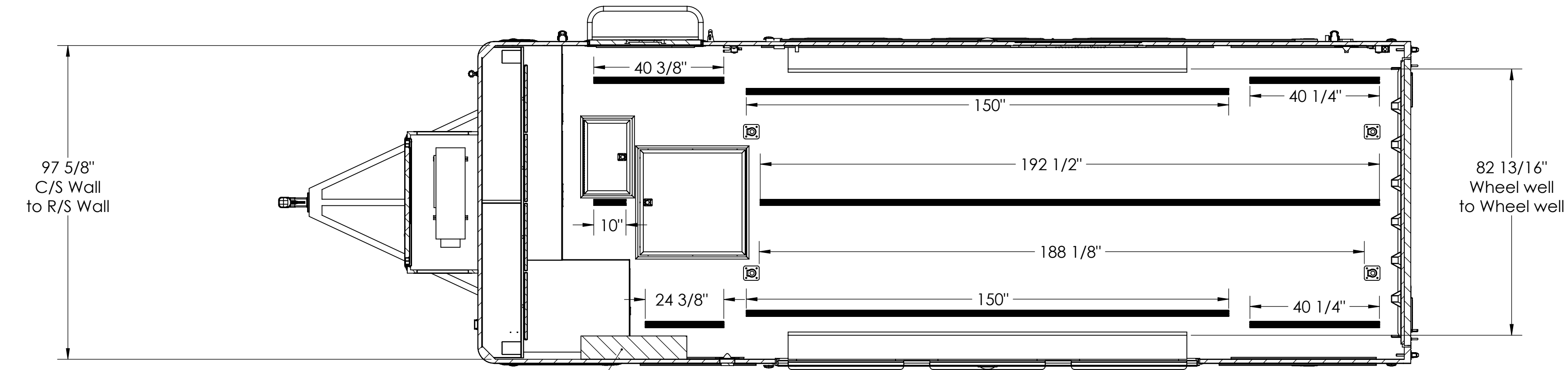
TOP VIEW POPULAR OPTIONS FLOOR LAYOUT SECTION J-J SCALE 1 : 26
