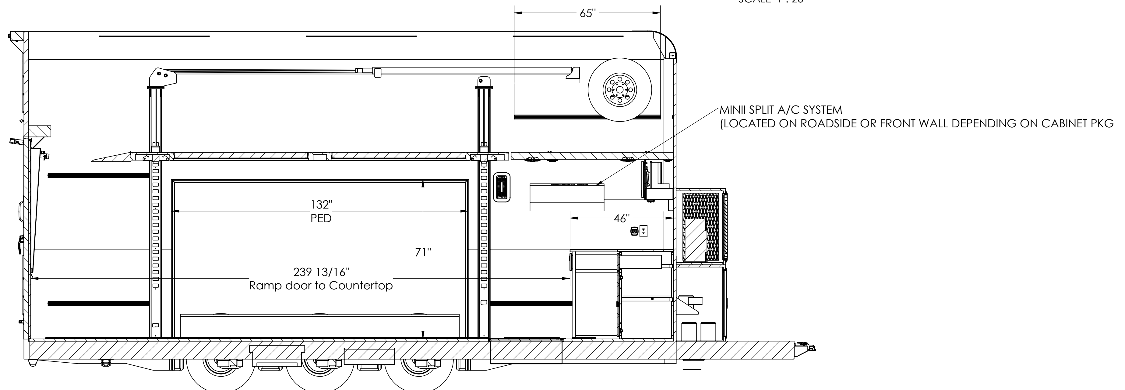
INTERIOR ROADSIDE VIEW SECTION G-G SCALE 1 : 26
