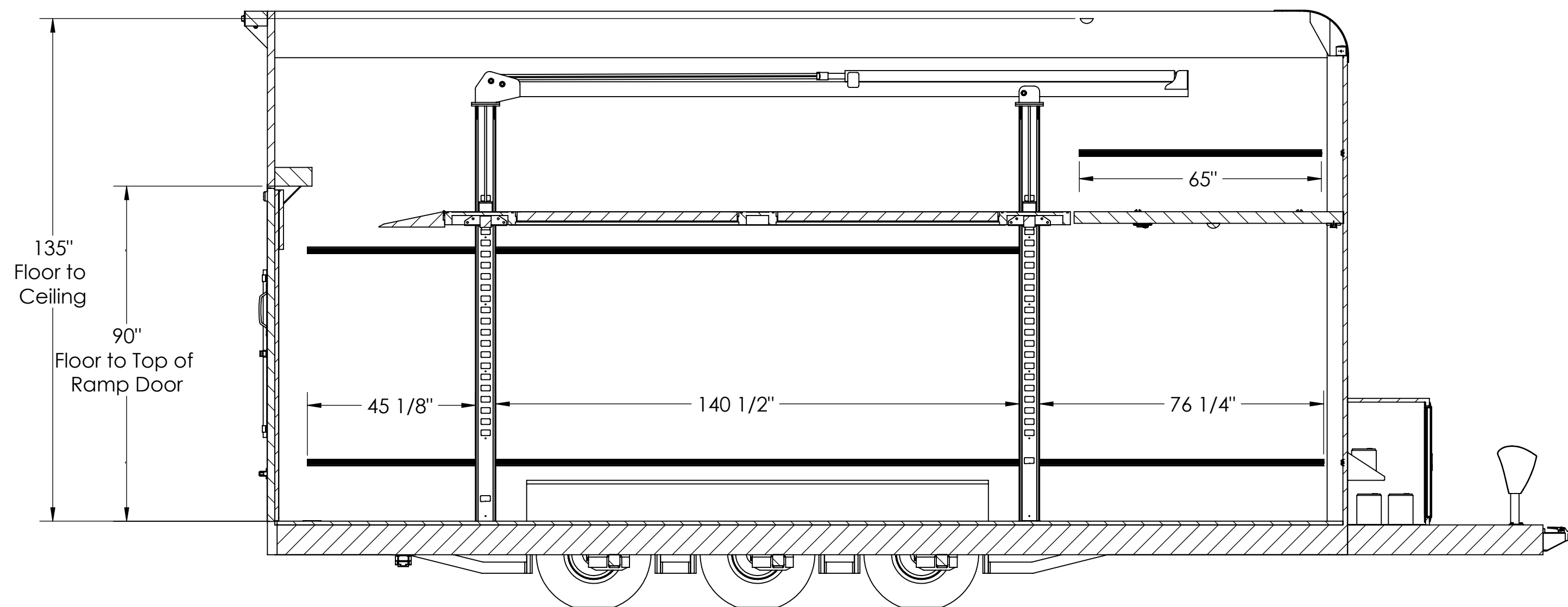
SECTION B-B
