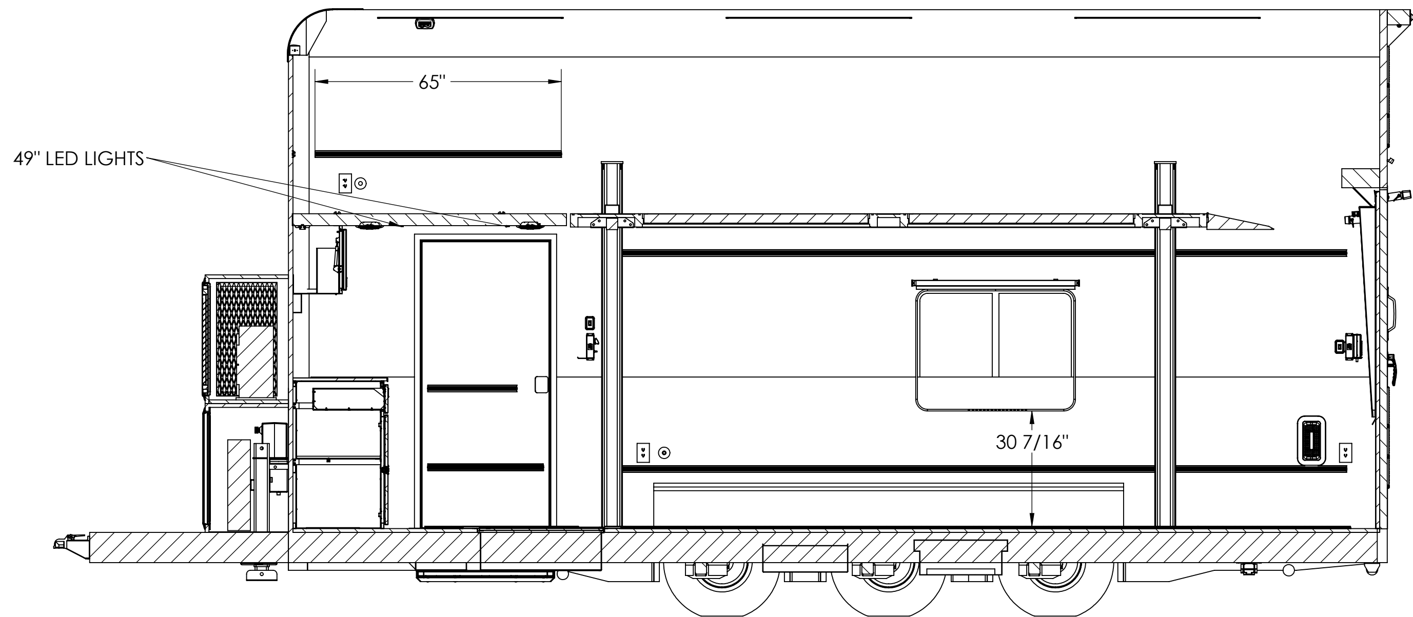
INTERIOR CURBSIDE VIEW SECTION F-F SCALE 1 : 26
